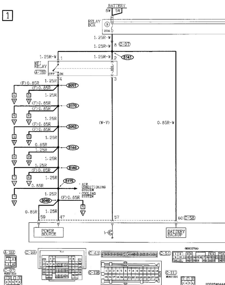
MFI System - M/T (With Variable Induction Control (VIC) System) Part 1
