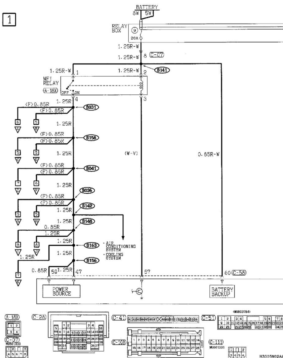
MFI System - M/T (Without Variable Induction Control (VIC) System) Part 1
