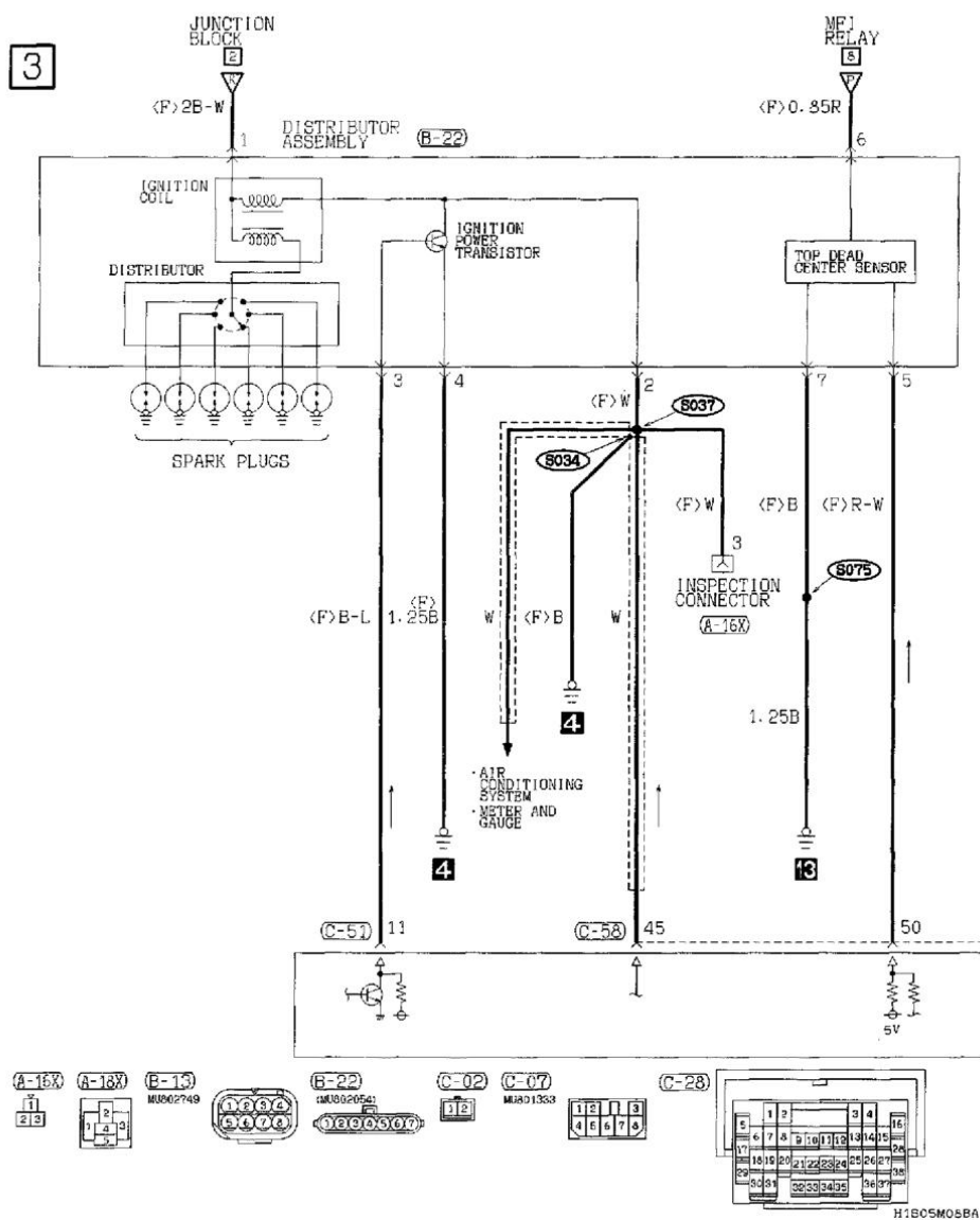
MFI System <3.0L Engine-M/T> Part 3
