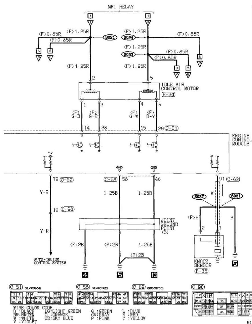
MF1 System &lt;3.0L Engine-M/T&gt; Part 8
