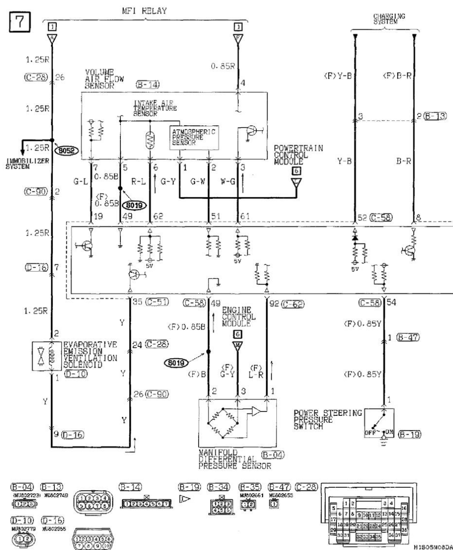
MFI System <3.0L Engine-M/T> Part 7
