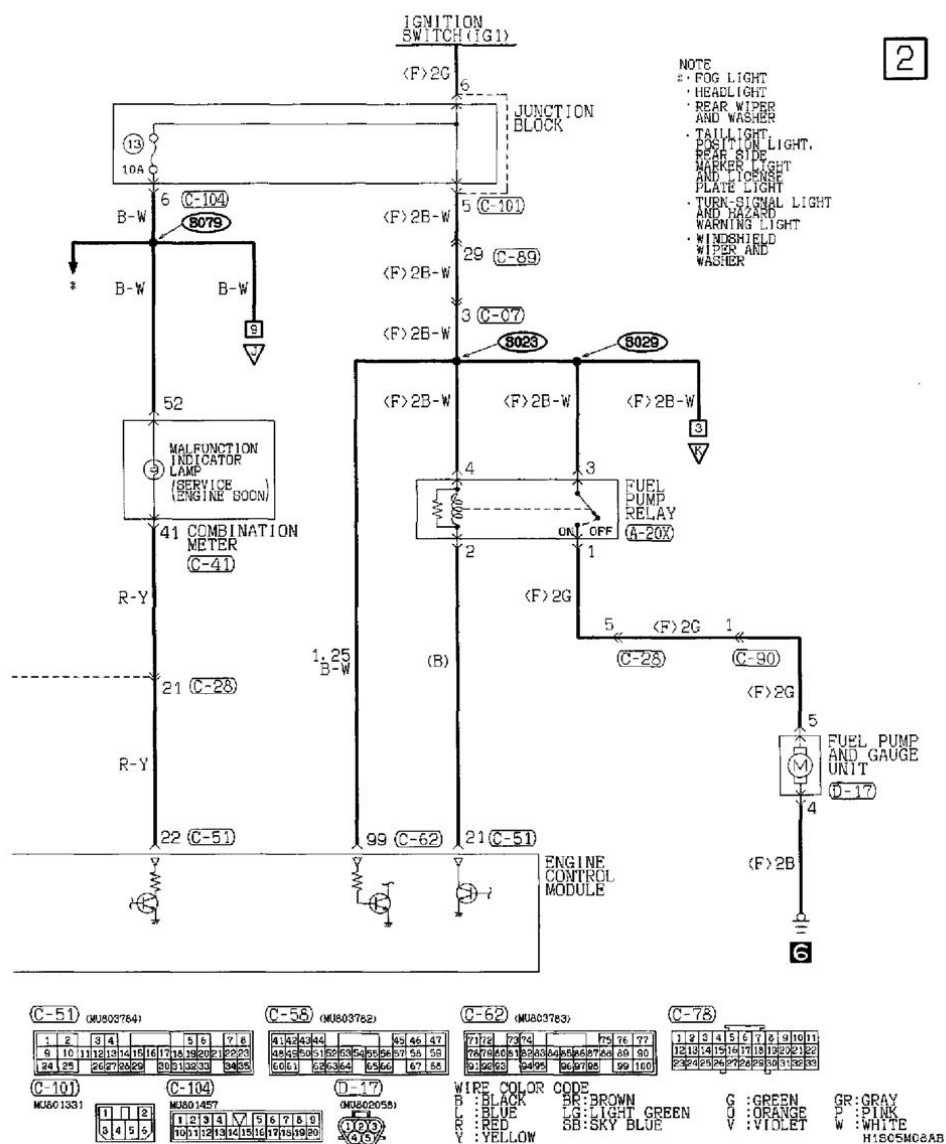
MFI System <3.0L Engine-M/T> Part 2
