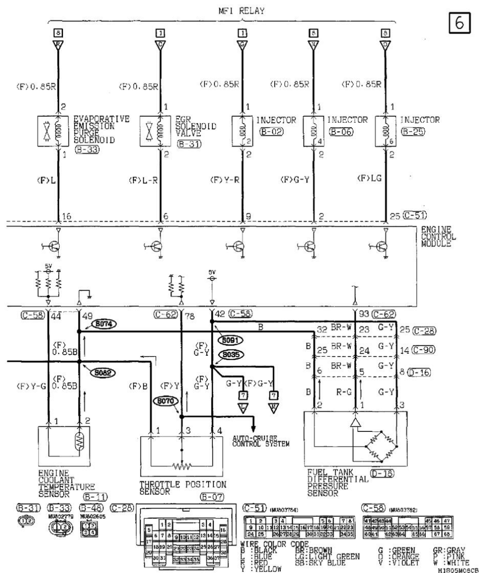
MFI System &lt;3.0L Engine-M/T&gt; Part 6
