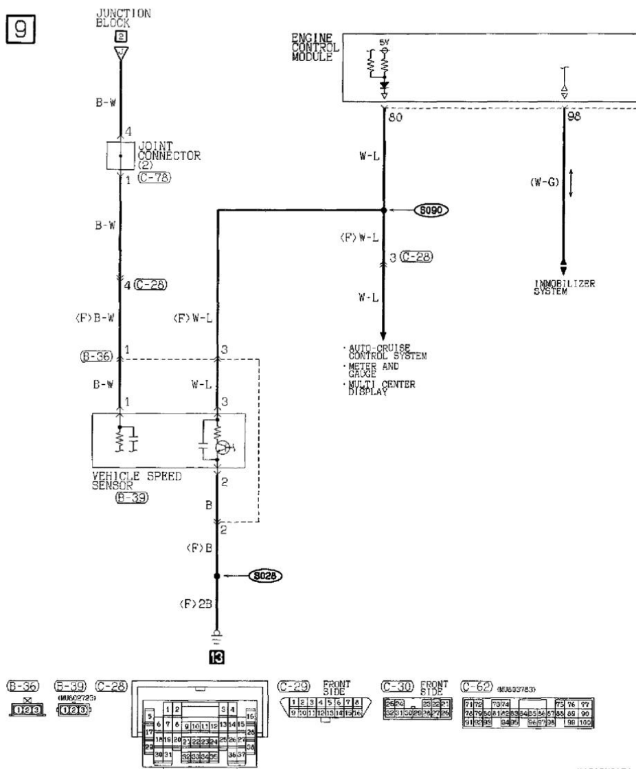
MFI System &lt;3.0L Engine-M/T&gt; Part 9
